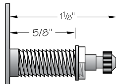
980.883 (Old #M88LCP) Long Post for Dials up to 5/8'' Thick.
