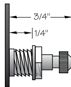
980.909 No Pendulum. Regular post for Dials up to 5/16".
