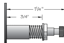
980.910 No Pendulum. Long post for Dials up to 3/4".
