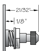
980.881 (Old #M88SP) Short Post for Dials up to 1/8'' Thick.
