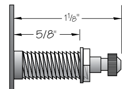
980.893 (Old #M89LCP) for Dials up to 5/8" Thick.
