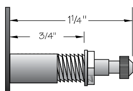
980.903 for Dials up to 3/4" Thick.
