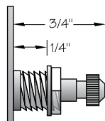
980.882 (Old #M88) Medium Post for Dials up to 1/4'' Thick.
