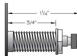
980.813 (Old #M81LCP) for Dials up to 3/4'' Thick.
