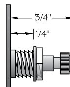
980.892 (Old #M89) for Dials up to 1/4" Thick.
